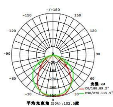
S1610A distribution curve flux effective mean
